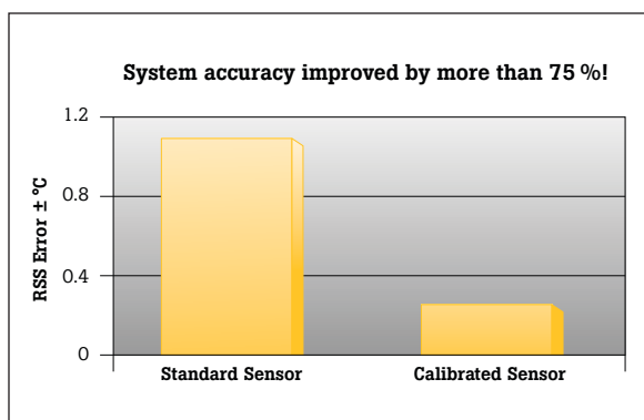
Figure 3. System accuracy improvement achieved with a calibrated Pt100 Sensor.
