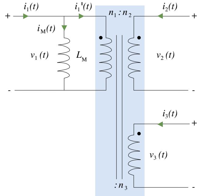
Ideal Transformer
