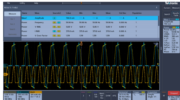
Figure 11. Power Quality Measurements.
