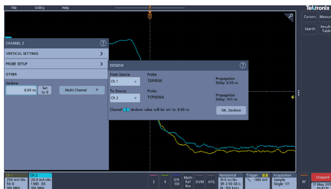
Figure 6. Nominal Correction of Timing Skew between Voltage and Current Probes.
