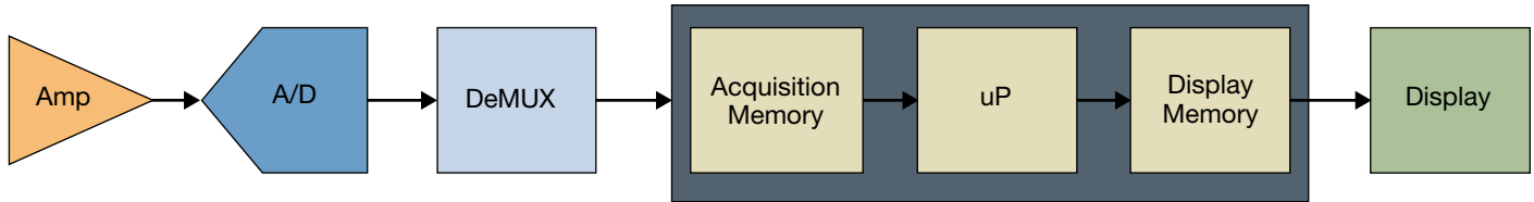
Figure 4. Serial-processing architecture of a digital storage oscilloscope (DSO).
