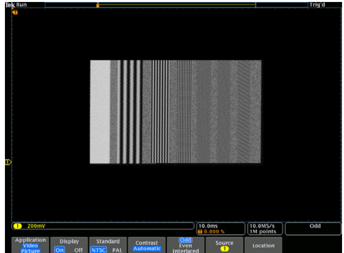
Figure 15. Video picture display of an NTSC multiburst signal.
