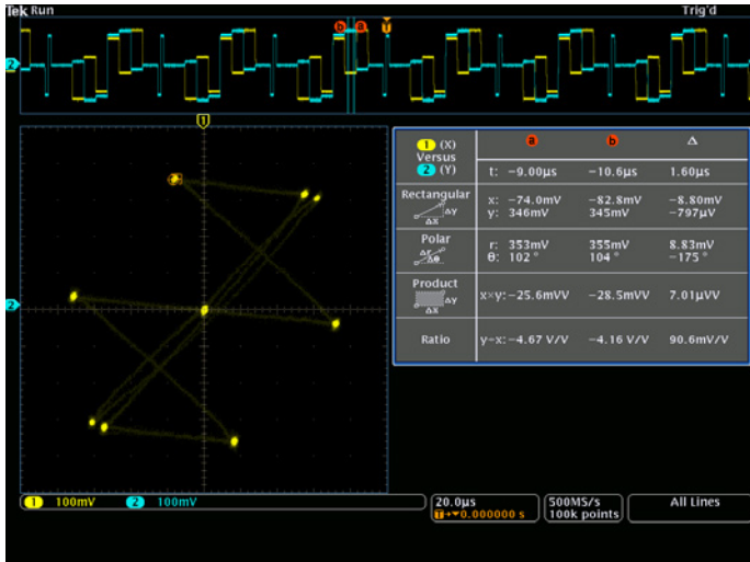
Figure 14. The 4000 Series' XY mode used to view a vectorscope-like display of chroma component signals. Screen cursors with polar readouts indicate the magnitude and phase of the red vector.
