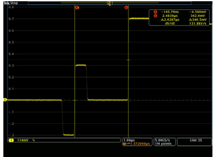
Figure 10. Using cursors to measure the Y signal white level amplitude and the time from 0H to the start of active video in a 1080i/60 HDTV 100% color bar signal.
