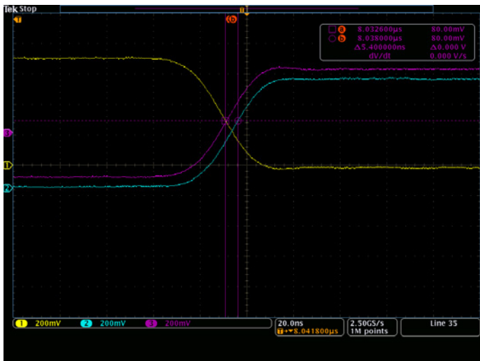
Figure 12b. Measuring the delay in the Pb signal due to an additional length of cable or processing time.
