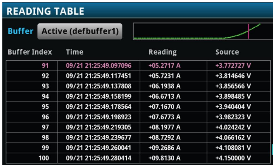
Figure 54: Reading table showing measurement results
