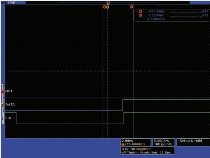
Figure 22. Triggering on the D-Flip-Flop data changing in the setup/hold window between cursor 'a' and 'b' around the rising clock edge.
