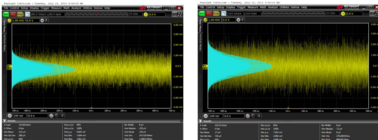
Figure 9. Noise performance comparison of Keysight DSA634A oscilloscope channels (standard vs “RealEdge”) showing 29% higher noise on RealEdge channel
