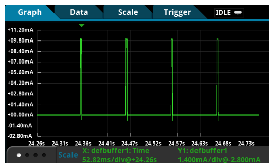
Repetitive device operation over a long time
