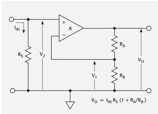
Shunt Ammeter
