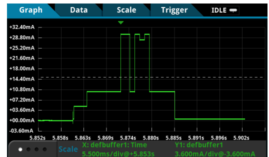
Device operating in a wide dynamic range
