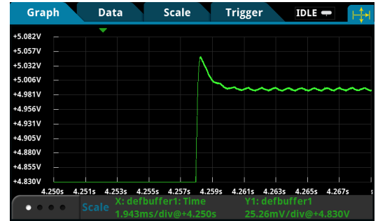
Analog measurement bandwidth
