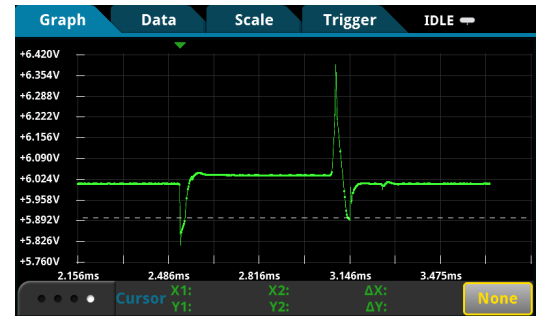
Fast response to a large load change
