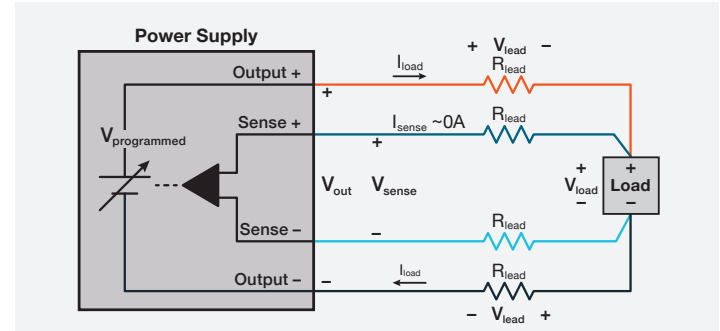
Ensure that the Programmed Voltage is Accurately Delivered to the Load
