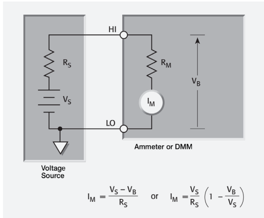
Effects of Voltage Burden on Current Measurement Accuracy
