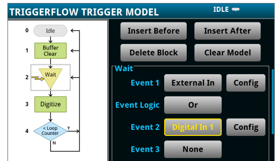
Advanced trigger
