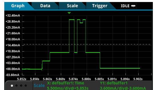
Transmit and receive current consumption profile
