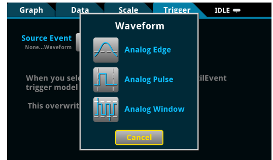
Built-in trigger options
