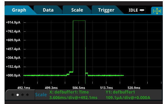
Ultra low level sleep current consumption
