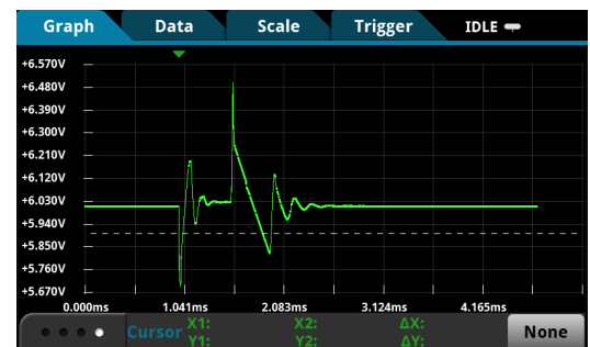
Poor response to a large load change
