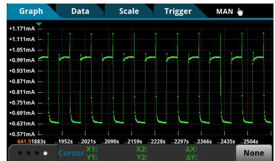
High-speed sample rate
