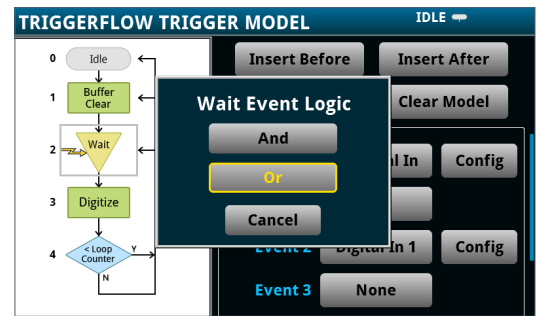
TriggerFlow enables logic trigger
