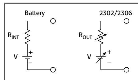
Figure 1. Simplified schematic of a battery and the 2302/2306.
