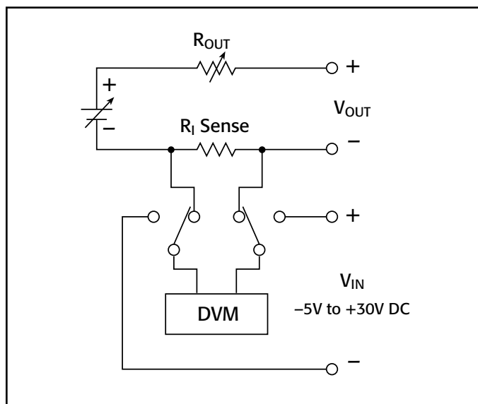
Figure 6. Model 2302 and Model 2306 Battery Channel Block Diagram. The Model 2306 charger channel is identical except it does not have the variable output resistance.
