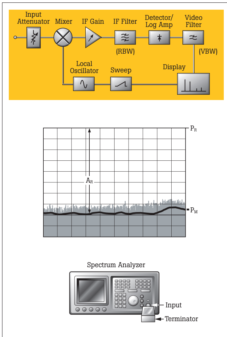
Figure 4. Noise Floor test and typical traditional equipment setup
