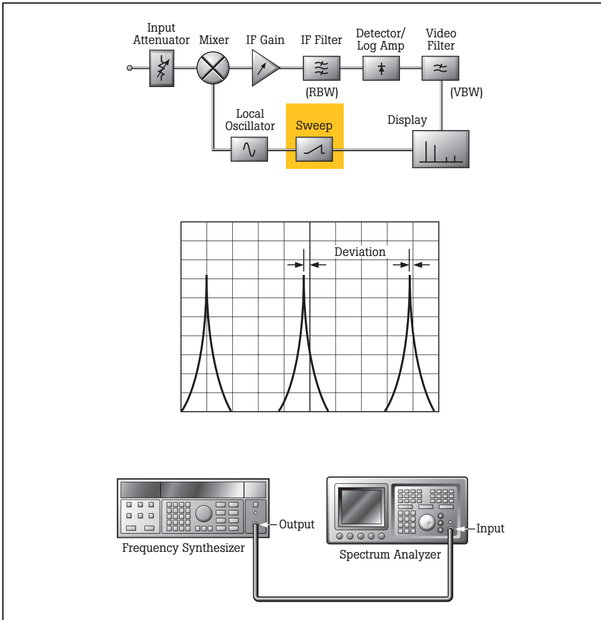
Figure 12. Frequency Span test and typical traditional equipment setup
