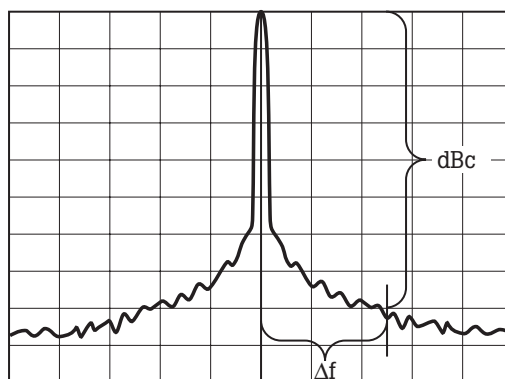
Noise level measurement at frequency offsets ( \Delta f ) above the carrier .
