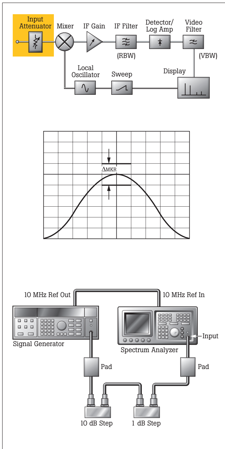
Figure 5. Input attenuator test and typical traditional equipment setup
