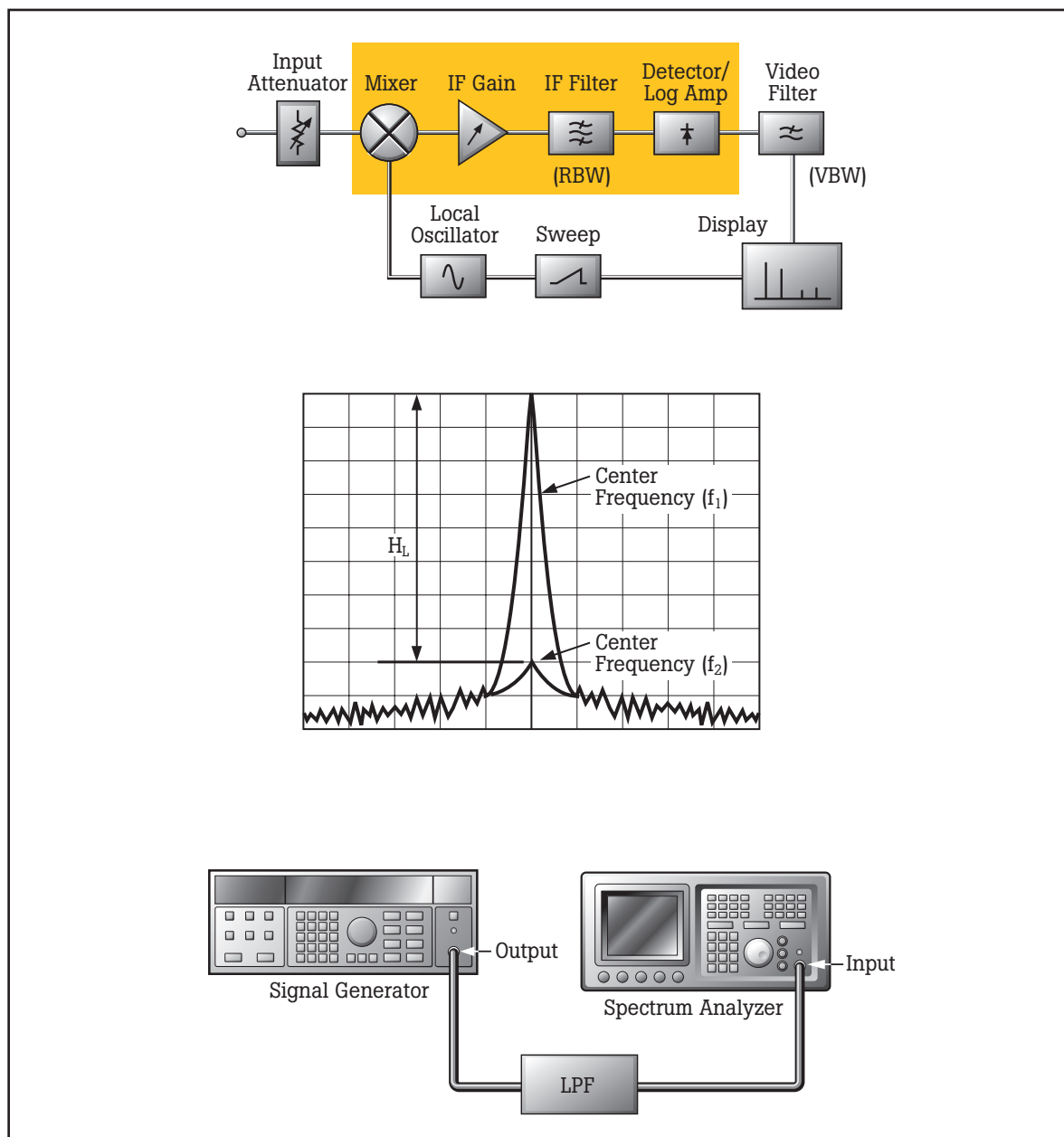
Fig 14. Harmonic Distortion test and typical traditional equipment setup
