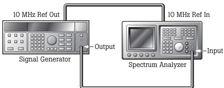
Figure 10. Noise Sideband test and typical traditional equipment setup
