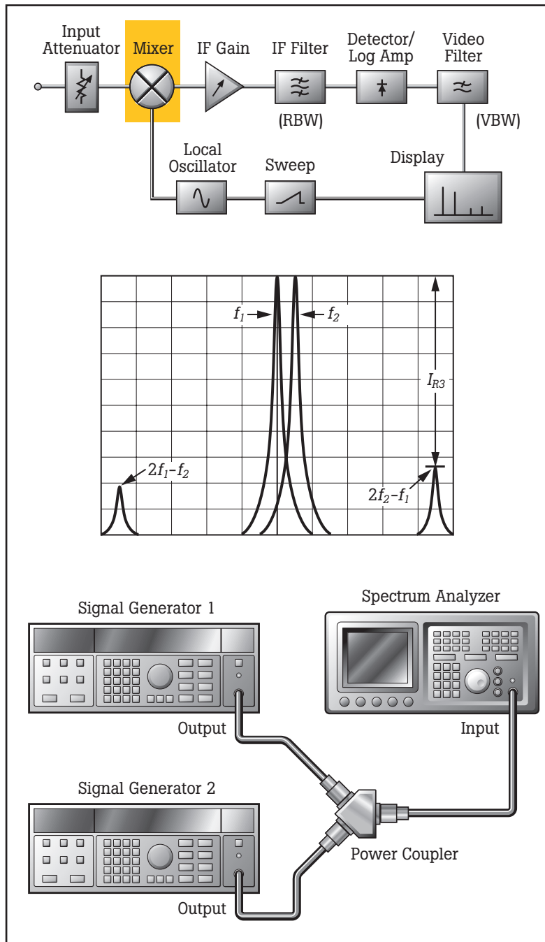
Figure 15. Third Order Intermodulation Intercept test and typical traditional equipment setup
