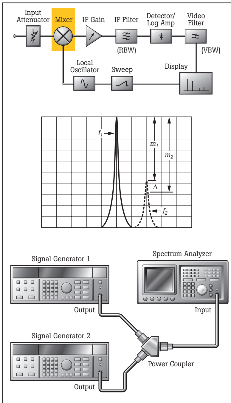
Figure 16. Gain Compression test and typical traditional equipment setup
