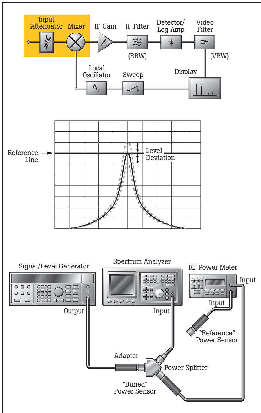
Figure 6. Frequency Response test and typical traditional equipment setup
