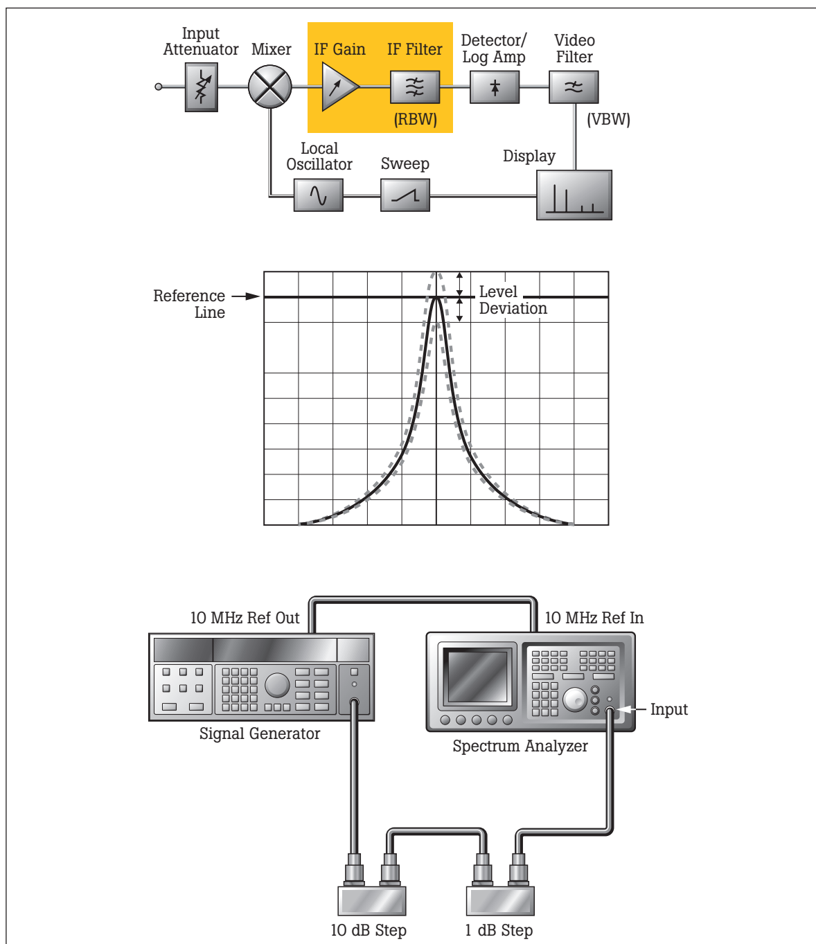
Figure 9. Reference Level Accuracy test and typical traditional equipment setup
