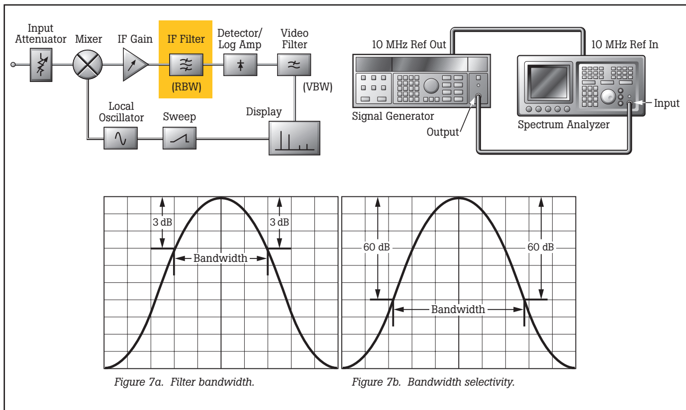
Figure 7. Resolution Filter Bandwidth and Selectivity test and typical traditional equipment setup
