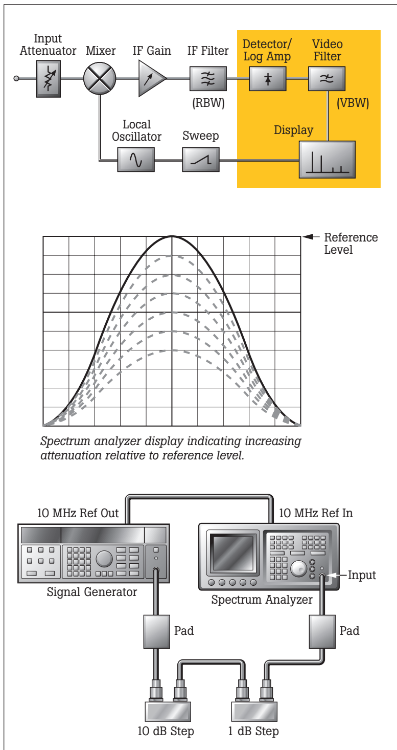
Figure 3. Display linearity test and typical traditional equipment setup
