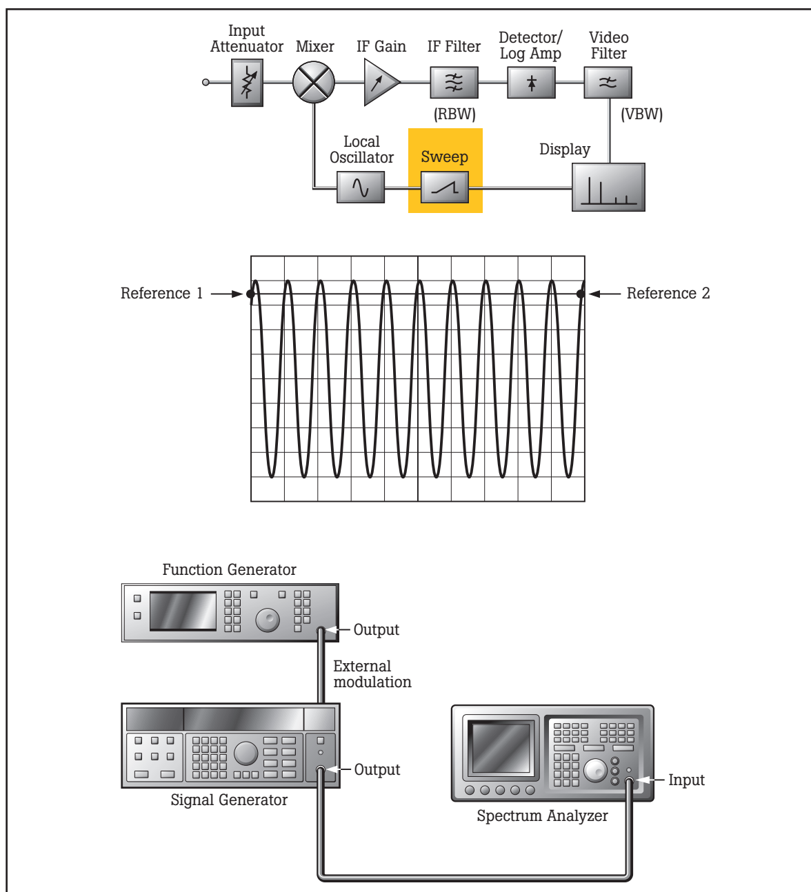
Figure 13. Sweep time accuracy test and typical traditional equipment setup
