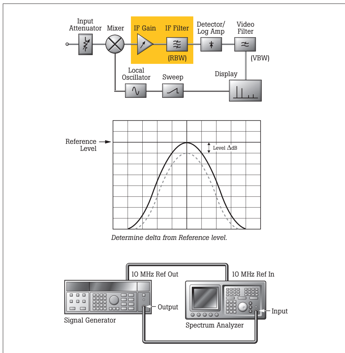
Figure 8. Resolution Bandwidth Switching test and typical traditional equipment setup
