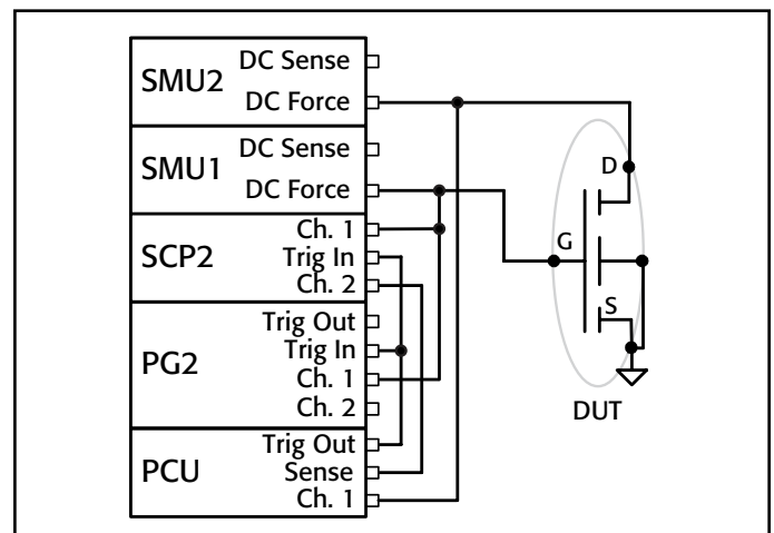
Interconnection for 4200-PIV-Q for III-V and LDMOS scaled-down RF transistors. PIV-Q pulses voltage on both the gate and drain from non-zero bias (quiescent) conditions.
