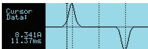
Acquired Current waveform (CSW Display).
