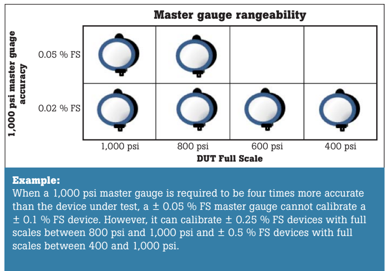
Figure 3. Rangeability of two 1,000 psi master gauges.
