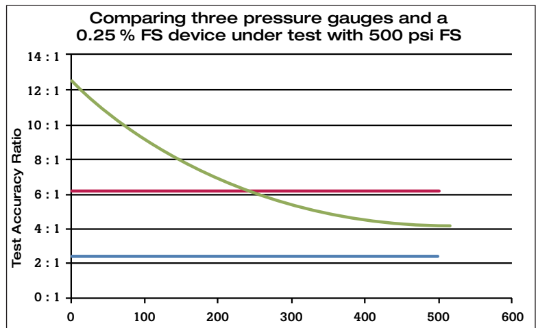
Figure 5. Comparing three pressure gauges and a device under test with 500 psi full scale.
