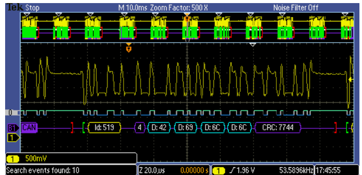
Search step 2: Wave Inspector automatically searches through the record and marks each event with a hollow white triangle. You can then use the Previous and Next buttons to jump from one event to the next.
