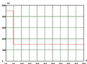
Pulse Current Measurement
