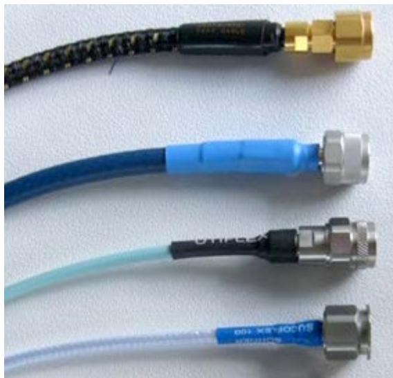
Figure 3. Precision metrology grade coaxial cables with N-Type connectors. Top two are level stable types.
